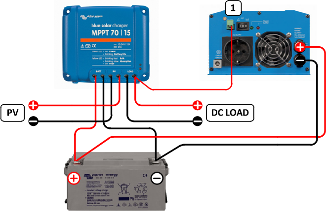
Figure 4: The Victron inverters model Phoenix 12/800, 24/800, 12/1200 and 24/1200 can be controlled by connecting the right side connection (1) of the inverter remote control directly to the solar charger load output
