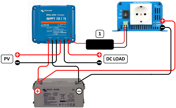
Figure 5: For the Victron inverters model Phoenix 12/180, 24/180, 12/350, 24/350, the Phoenix Inverter C models and the MultiPlus C models an interface cable (1) is needed (MPPT 70/15 to inverter remote on-off cable, article number ASS030550100)
